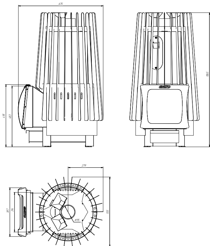
Fig. 1 Dimensions of heater Grill'D Cometa 180 Vega Short Window Max
